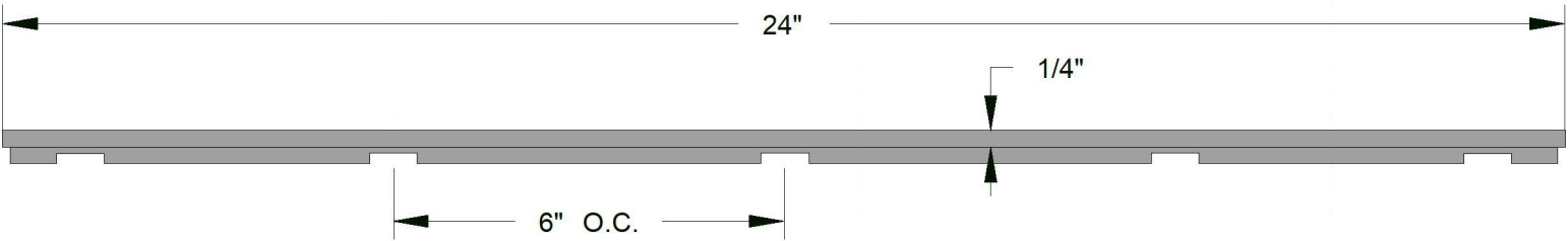
SIDE VIEW
