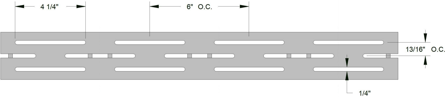
TOP VIEW
