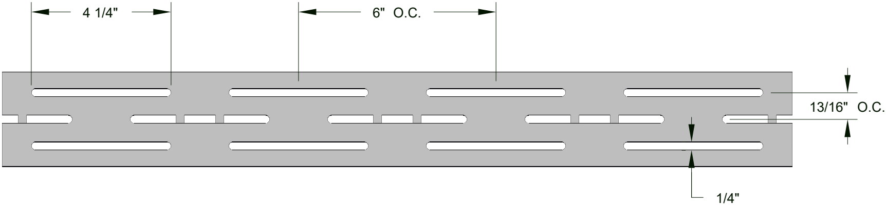
TOP VIEW
