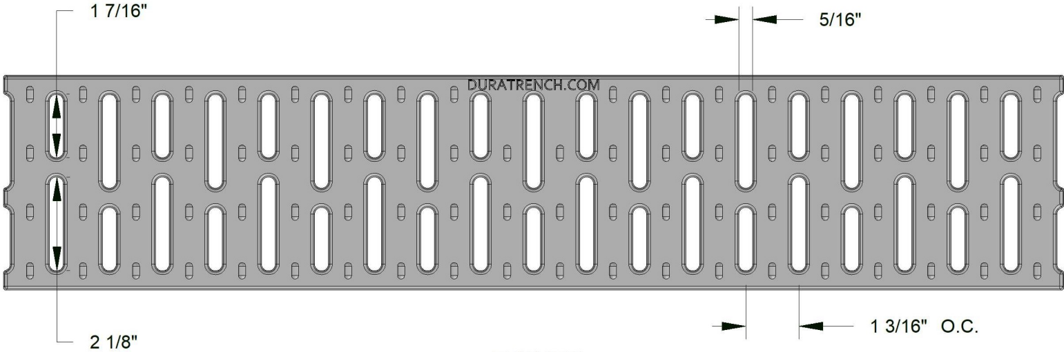
TOP VIEW
