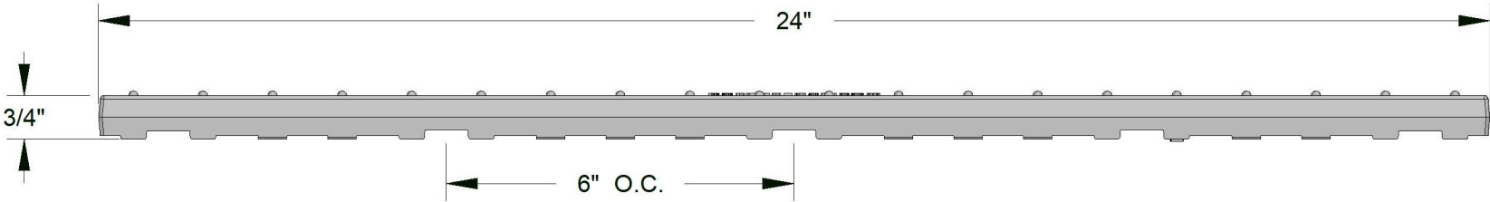
SIDE VIEW
