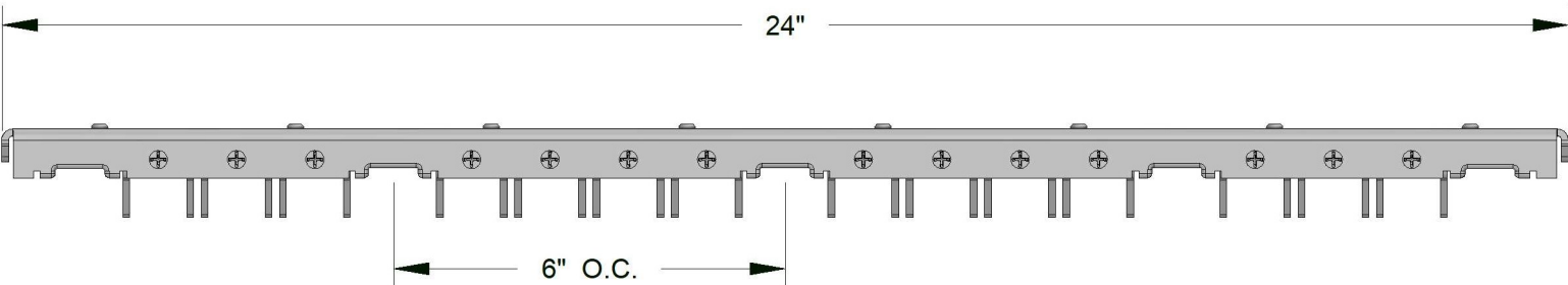
SIDE VIEW
