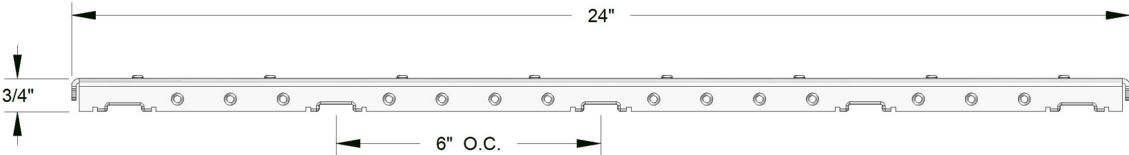
SIDE VIEW
