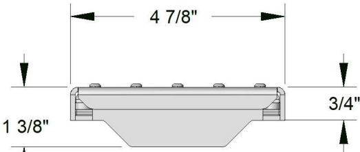
END VIEW
