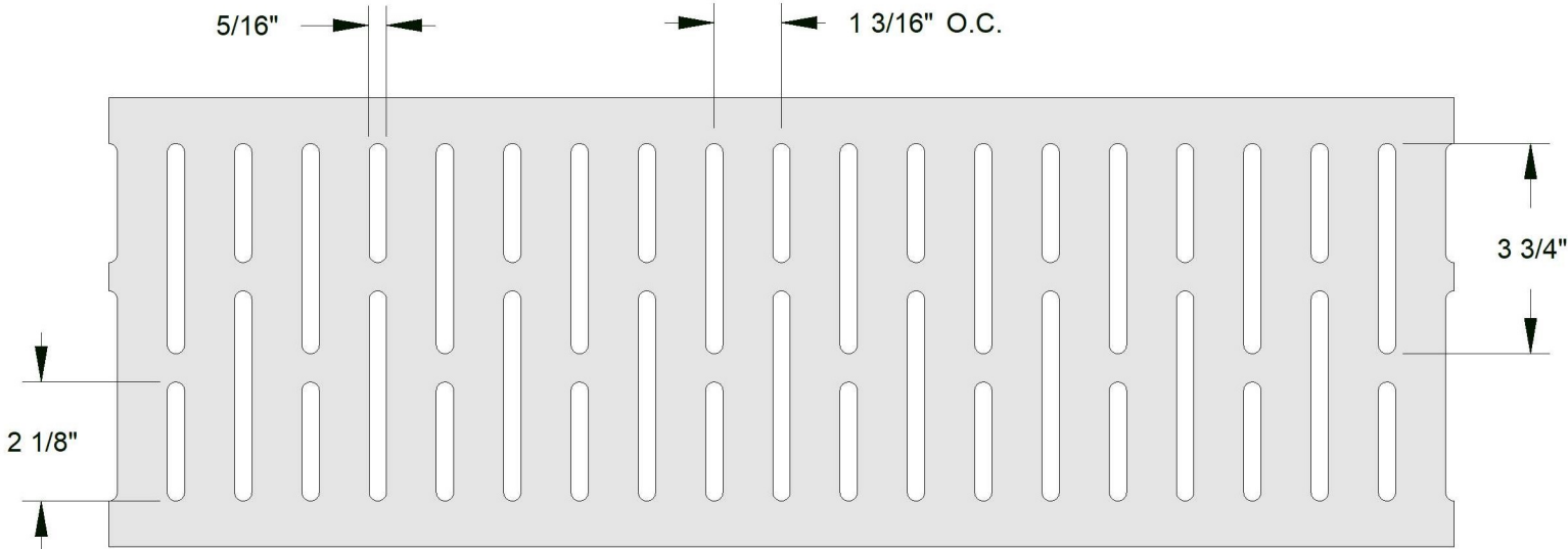
TOP VIEW
