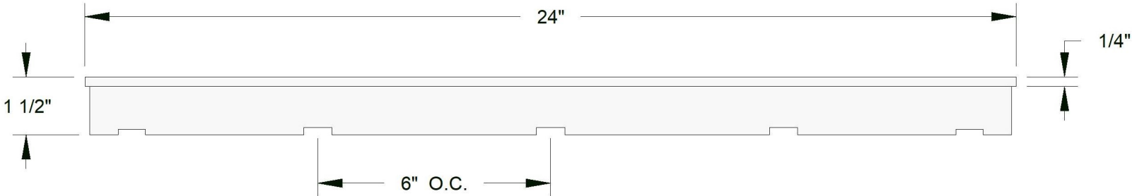
SIDE VIEW
