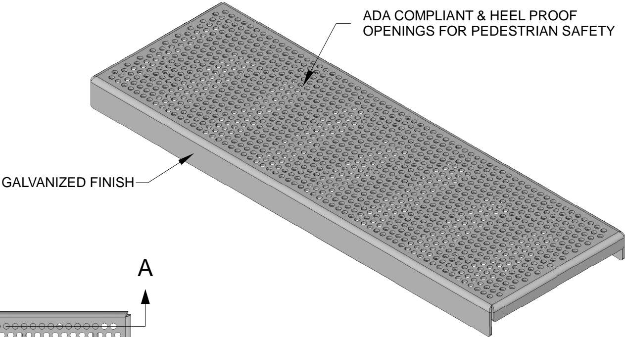
ISOMETRIC VIEW
