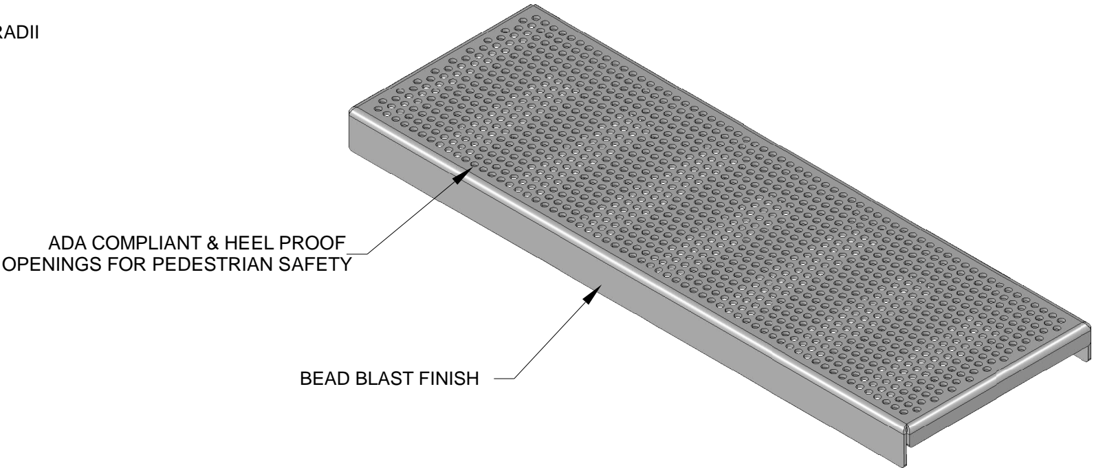
ISOMETRIC VIEW
