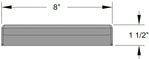
END VIEW
