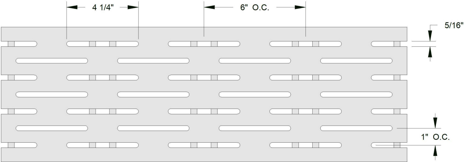
TOP VIEW
