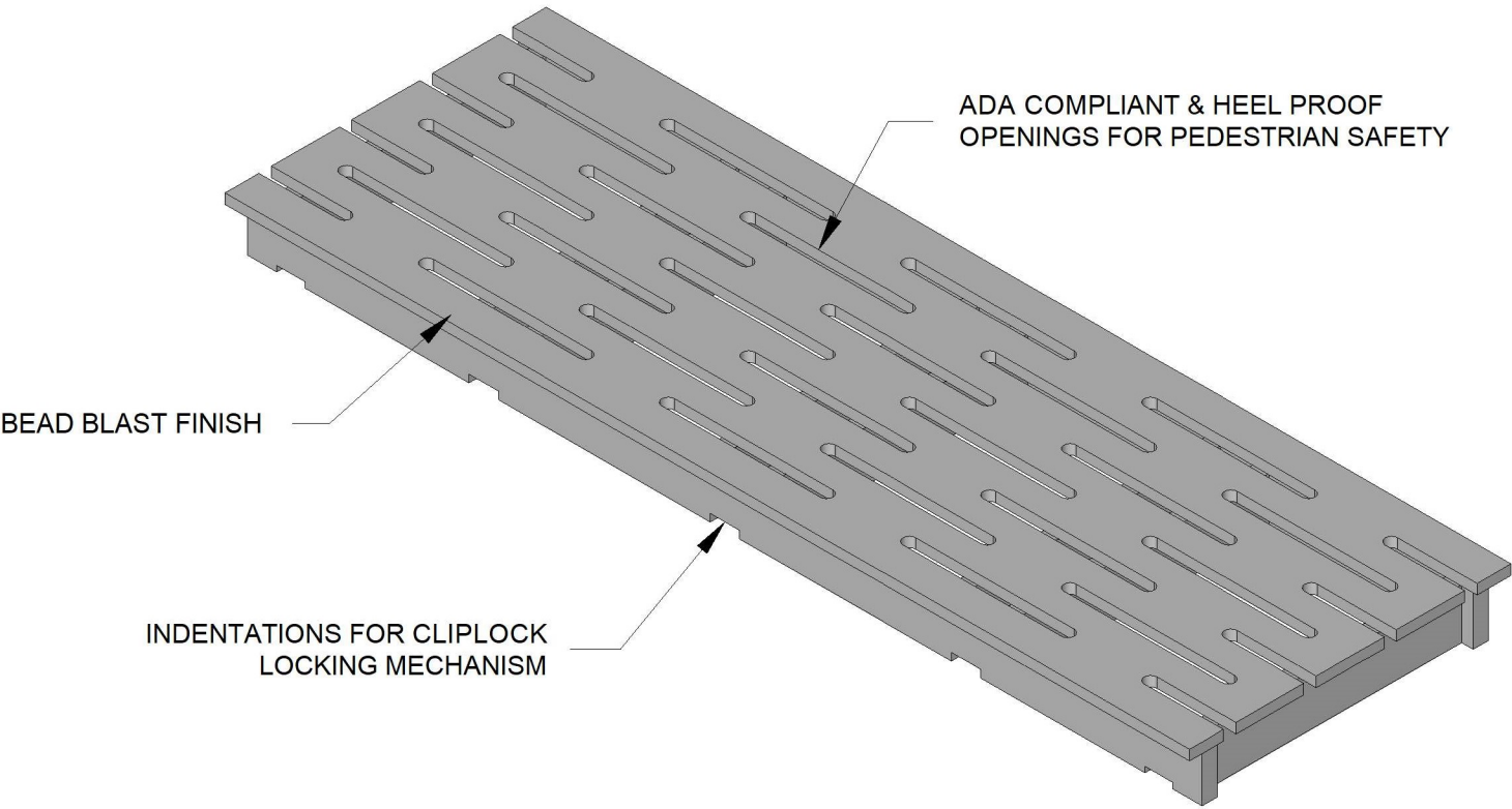
ISOMETRIC VIEW
