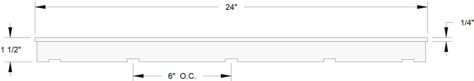
SIDE VIEW
