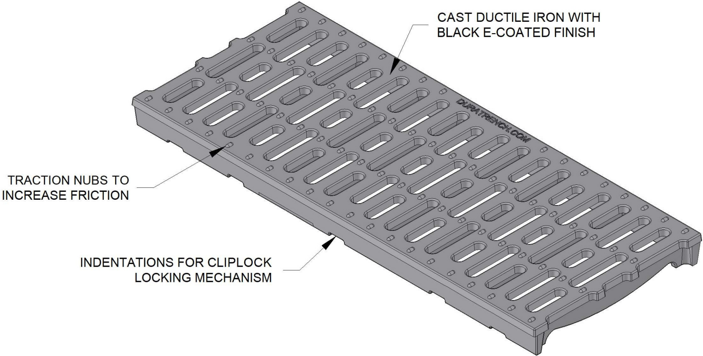
ISOMETRIC VIEW
