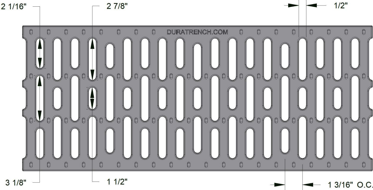
TOP VIEW
