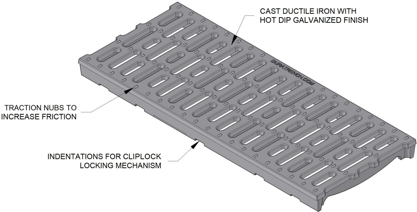
ISOMETRIC VIEW
