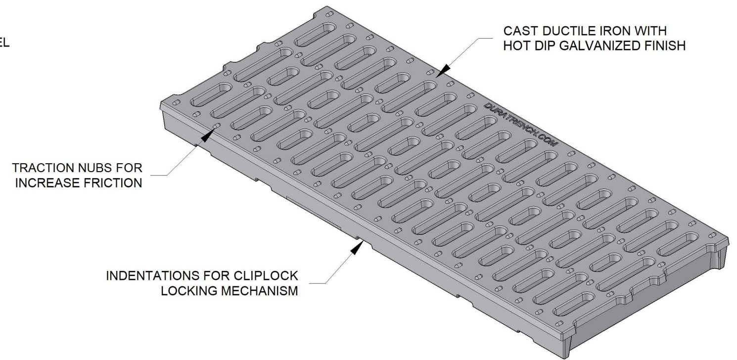
ISOMETRIC VIEW
