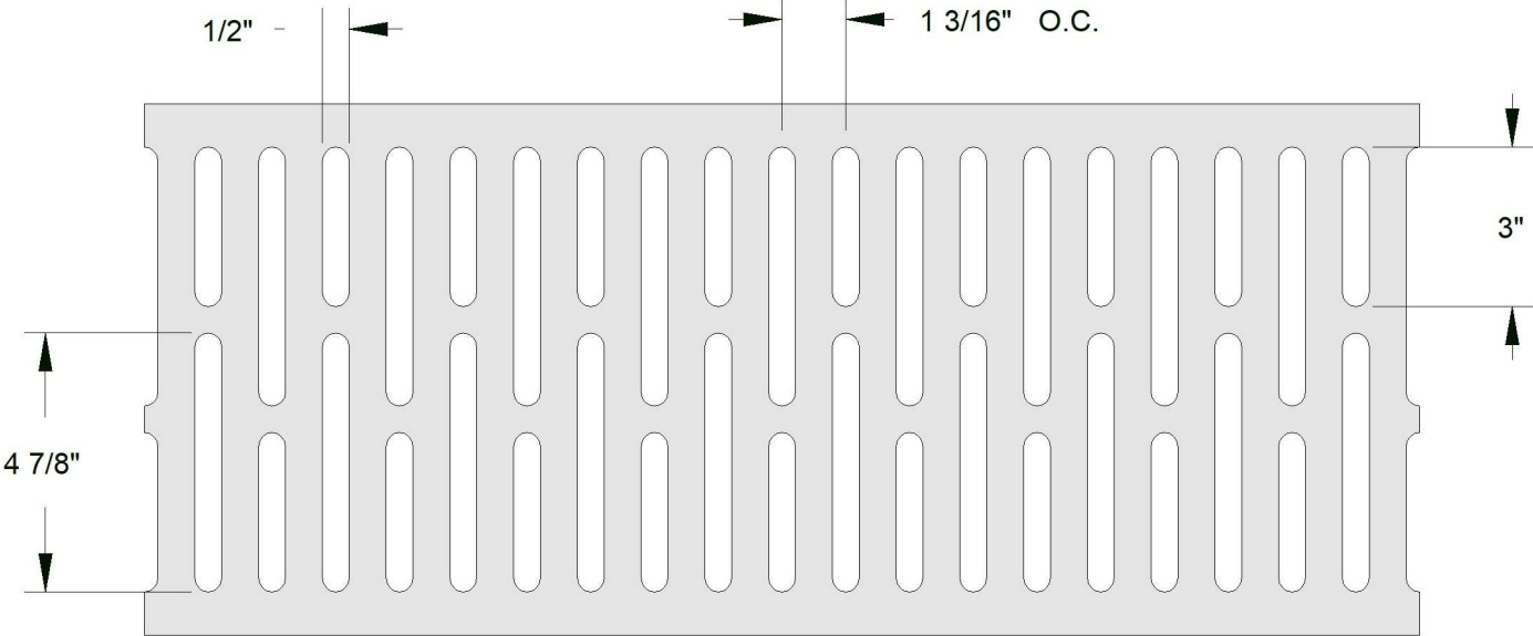
TOP VIEW
