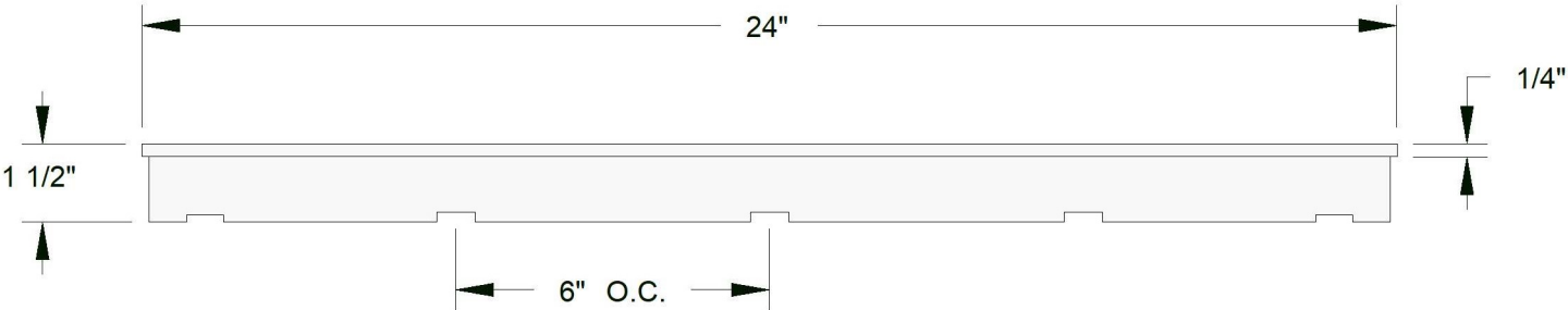
SIDE VIEW
