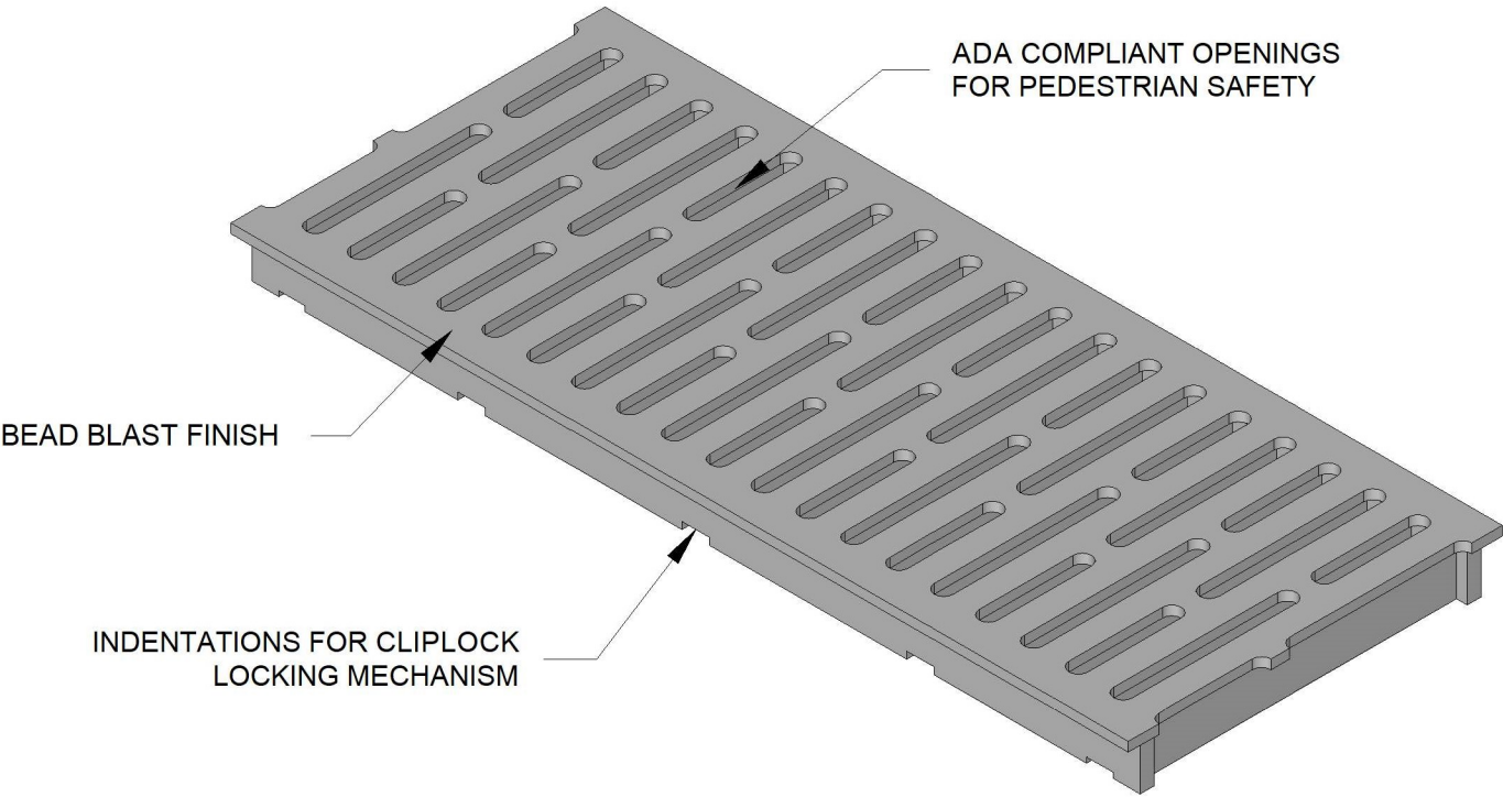
ISOMETRIC VIEW
