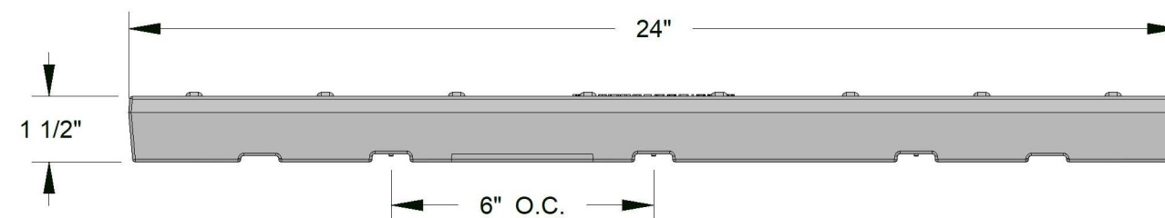
SIDE VIEW
