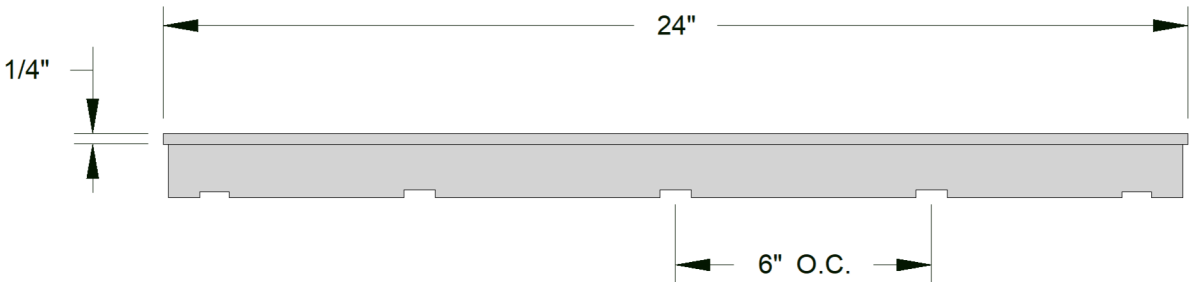
SIDE VIEW
