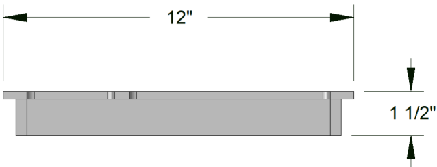
END VIEW
