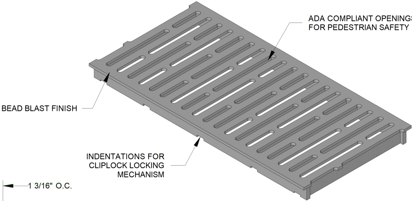
ISOMETRIC VIEW
