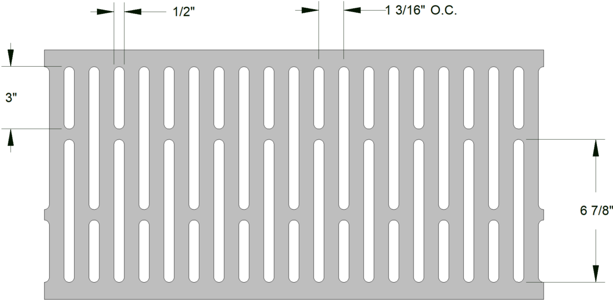
TOP VIEW
