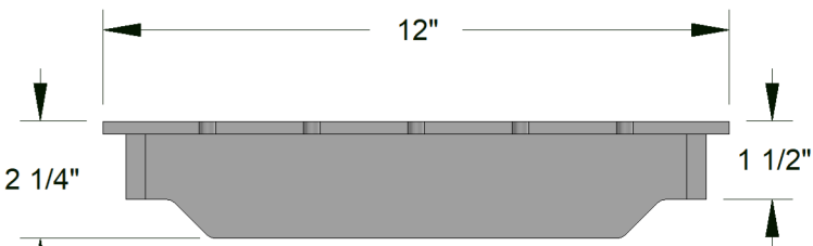
END VIEW
