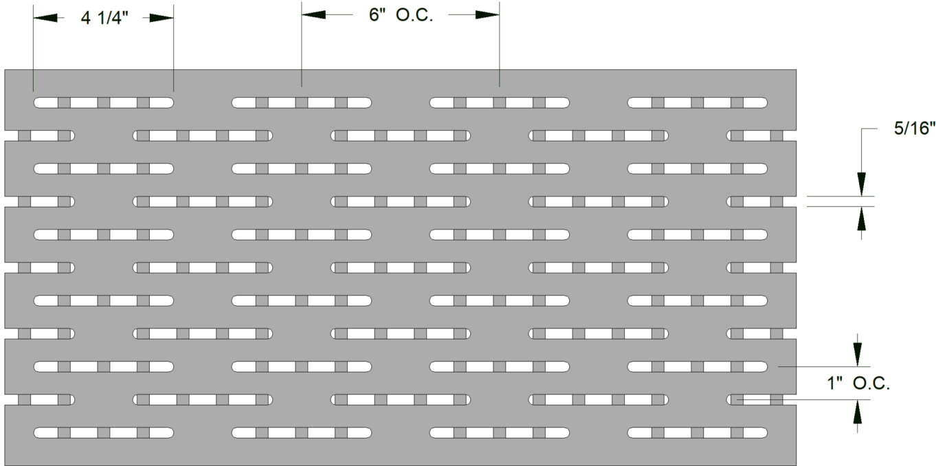
TOP VIEW
