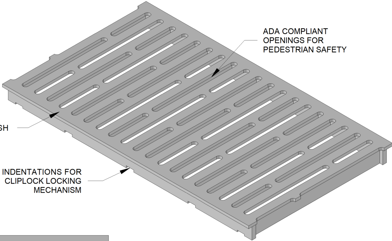
ISOMETRIC VIEW
