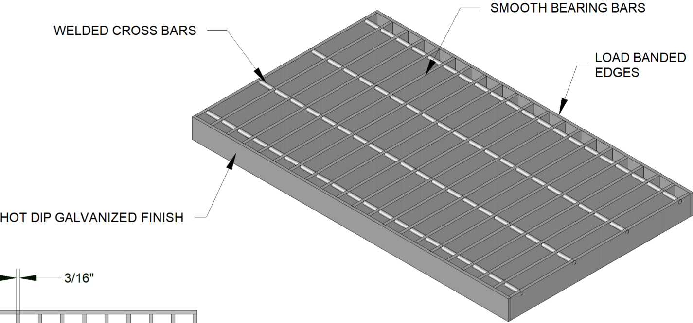
ISOMETRIC VIEW
