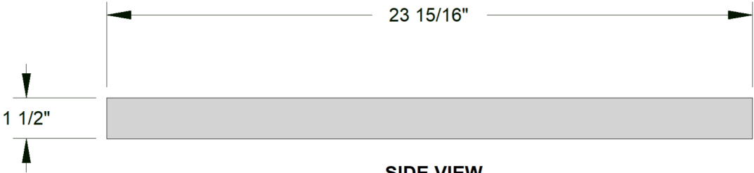
SIDE VIEW
