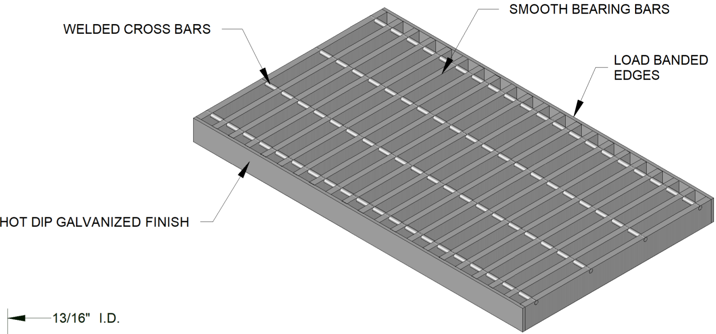
ISOMETRIC VIEW
