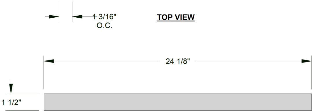
SIDE VIEW
