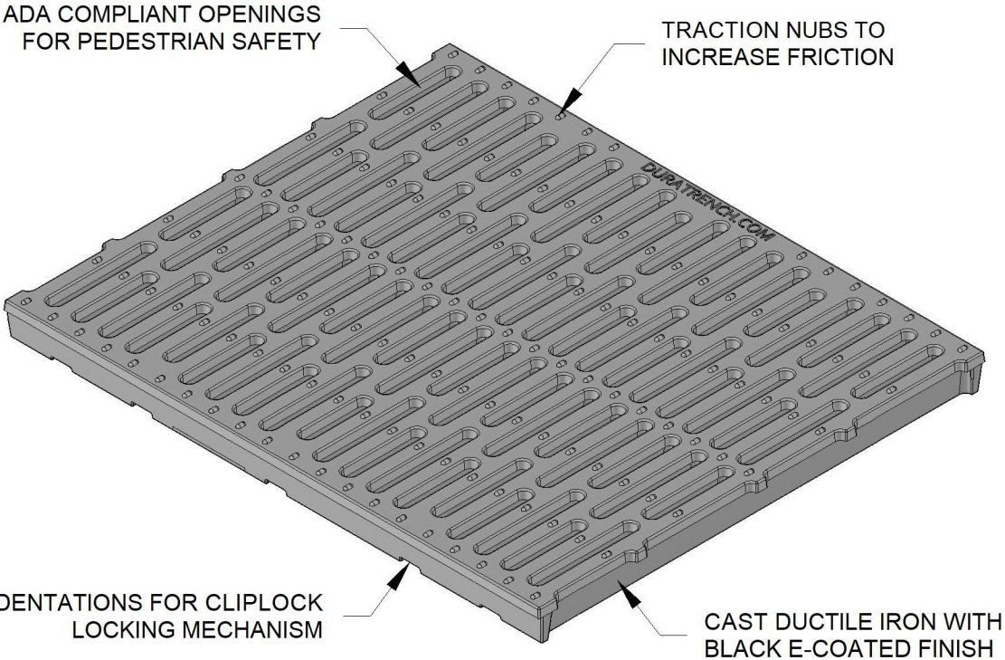
ISOMETRIC VIEW
