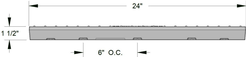
SIDE VIEW
