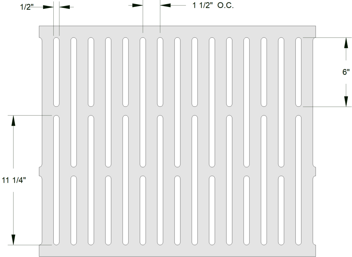
TOP VIEW
