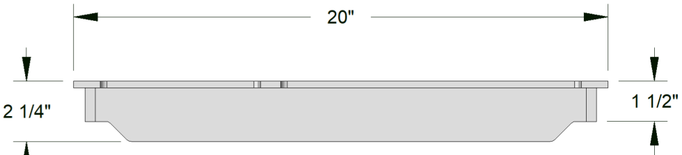
END VIEW
