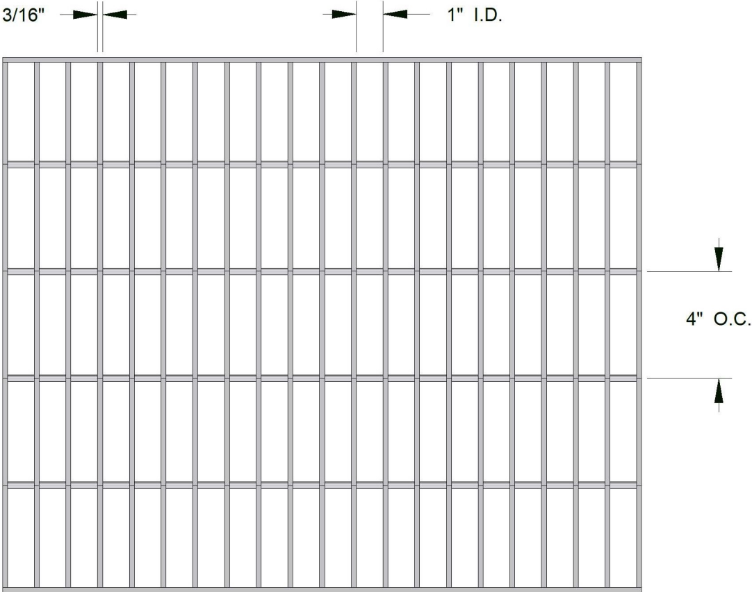
TOP VIEW
