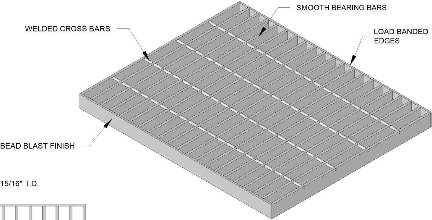
ISOMETRIC VIEW
