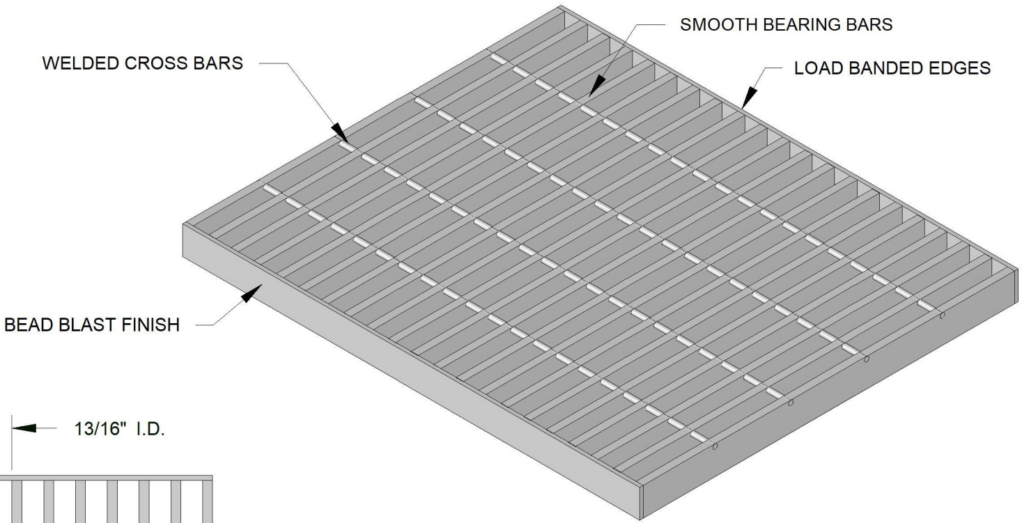
ISOMETRIC VIEW
