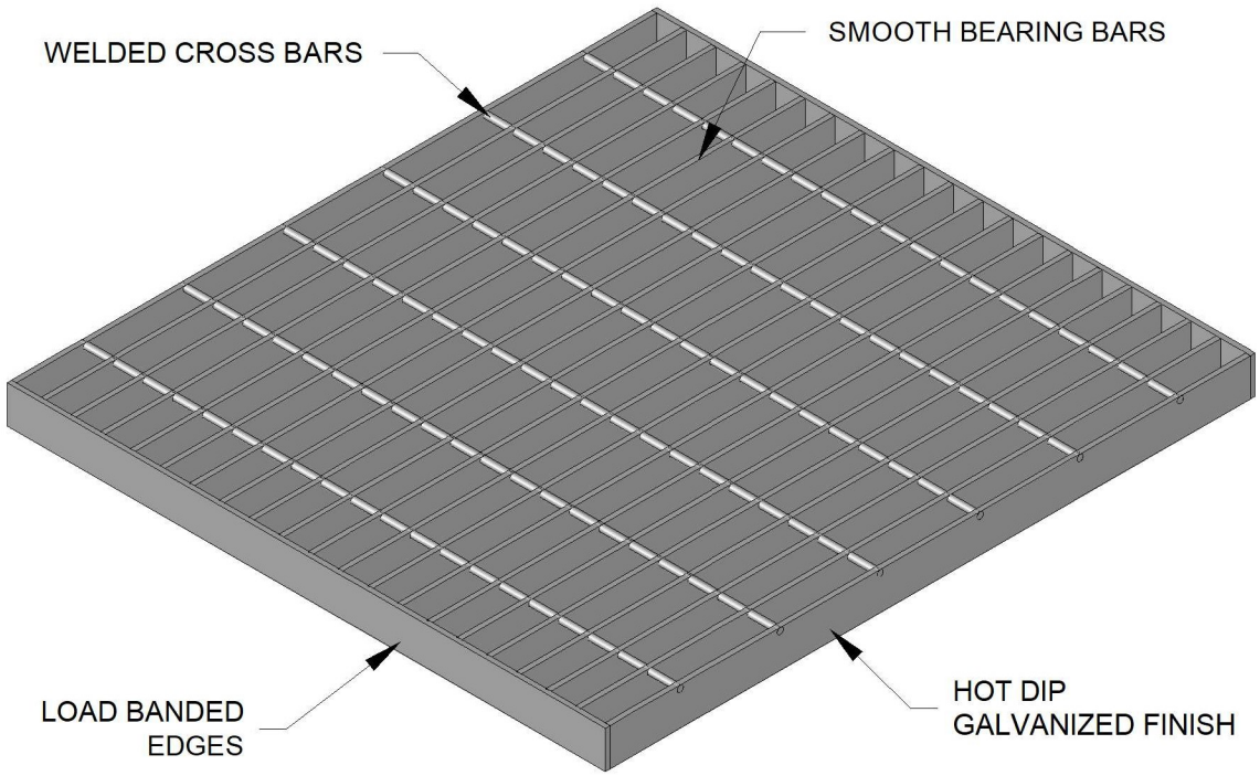
ISOMETRIC VIEW
