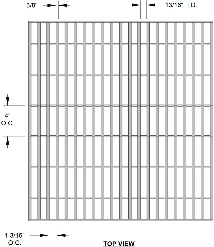
TOP VIEW
