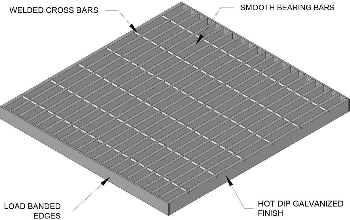
ISOMETRIC VIEW
