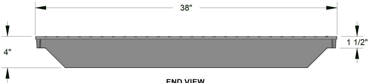
END VIEW
