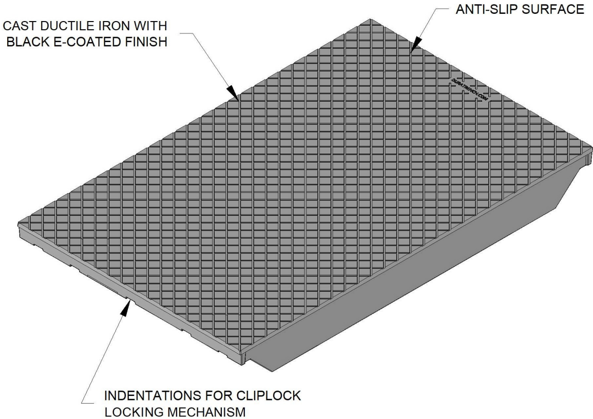
ISOMETRIC VIEW
