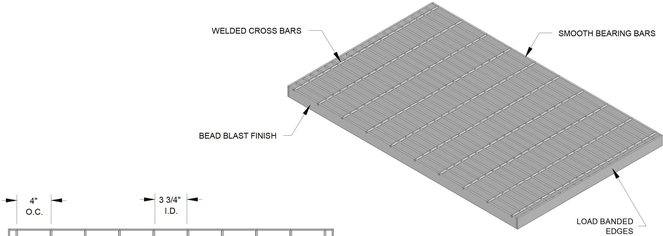
ISOMETRIC VIEW
