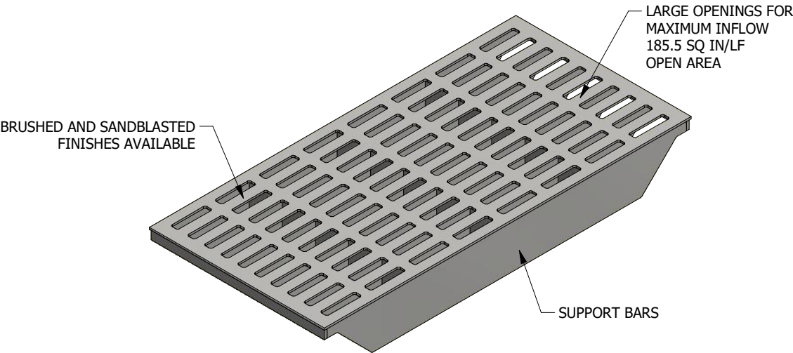
ISOMETRIC VIEW
