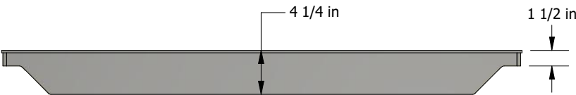
SIDE VIEW
