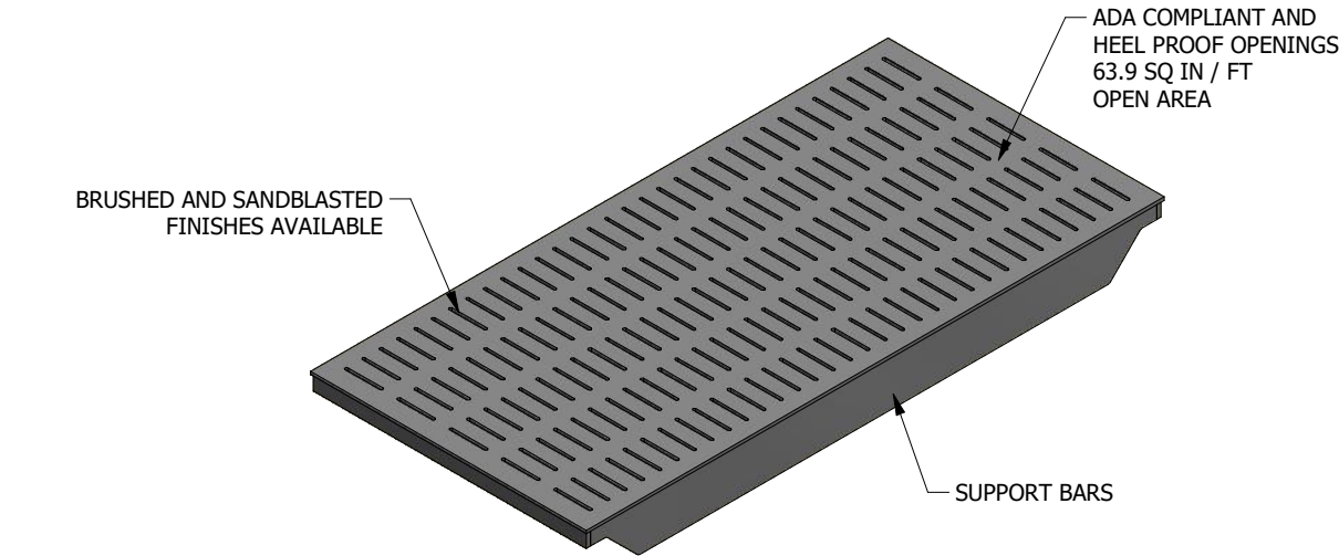
ISOMETRIC VIEW
